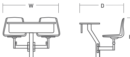
TAB - 100 1100W x 840D x 785H 440SH mm.
